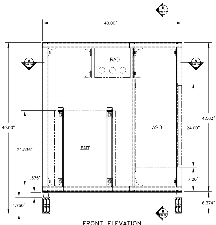
FRONT ELEVATION
