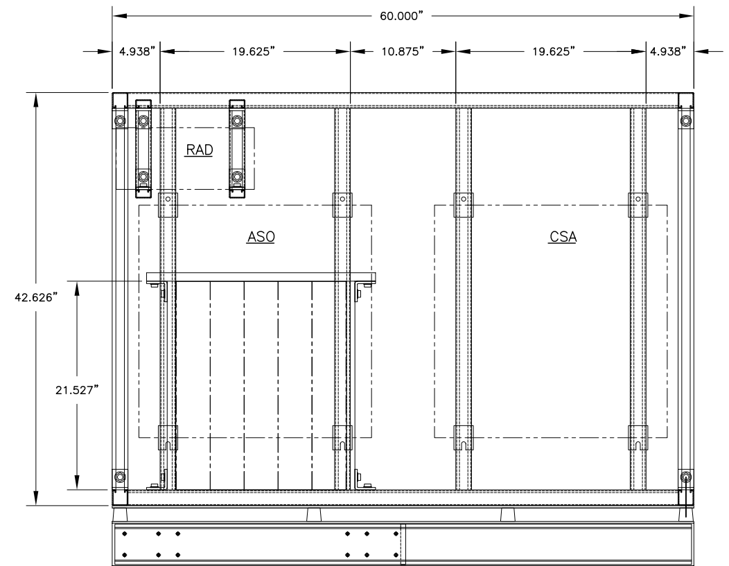
VIEW B-B
